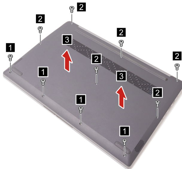
Figure 3. Remove 10 screws
